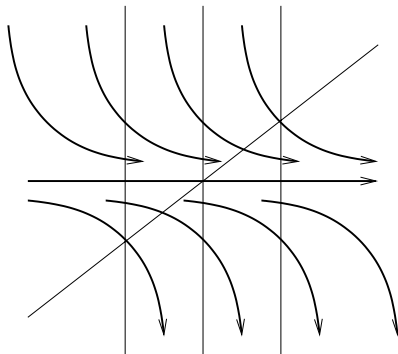
Figure 1. The flow of the field \dot{x} = -x^2 . The embeddings j_t are induced by the vertical slices. The completion is \bar{M} = \mathbb{R} , the identification is given by the inclined line, for example.
